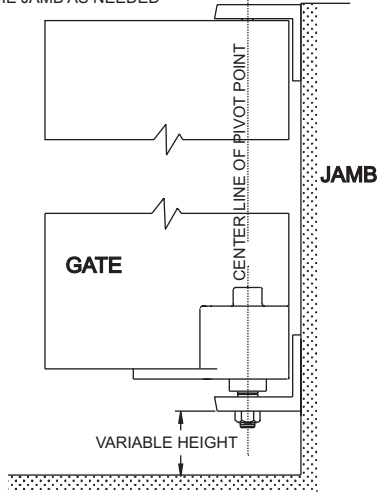
FLOOR STANDARD MORTISE PIVOT APPLICATION TO GATE AND JAMB
