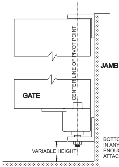
FLOOR STANDARD SURFACE PIVOT APPLICATION TO GATE AND JAMB
