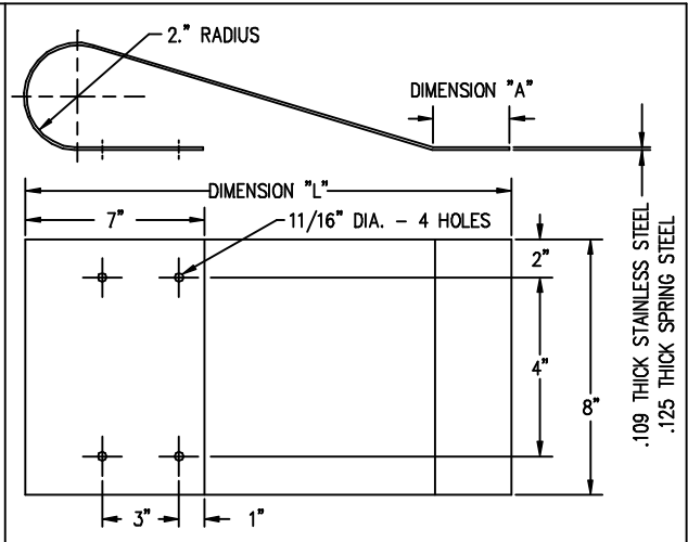
BUMPER
