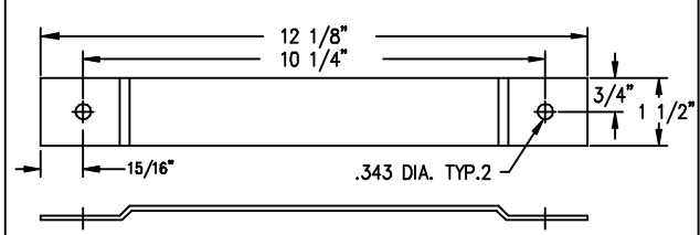
GUIDE PLATE
